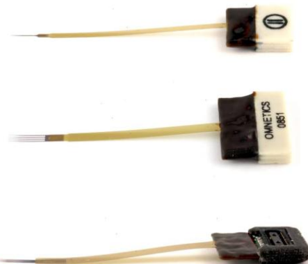
H16 / H32 / HZ64 Package F-Series replacement. Intended for use with microdrive systems.
